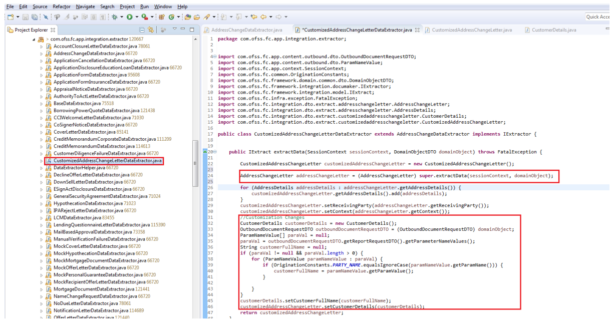
Figure 19–8 Customized AddressChangeLetterDataExtractor
