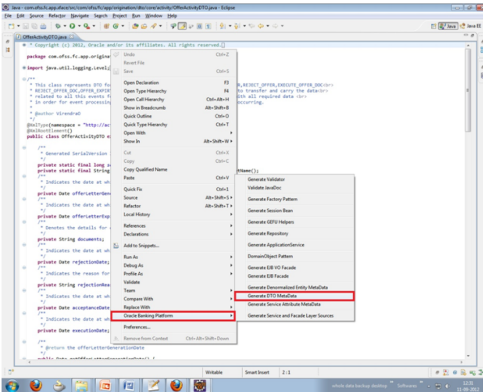
Figure 10–5 Metadata Generation
